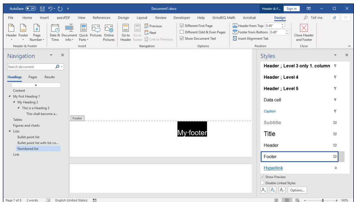
Figure 19: Edit footer
